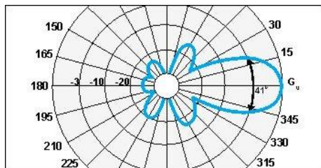
E-plane pattern Y6-4m
