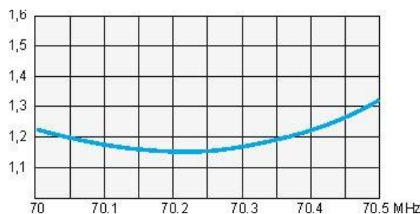
VSWR diagram Y6-4m
