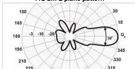
Y12-2m E-plane pattern
