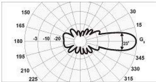
Y21-70cm E-plane pattern
