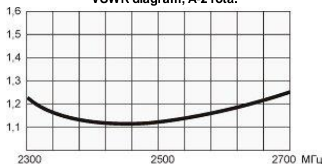
VSWR diagram, A-2Yota.
